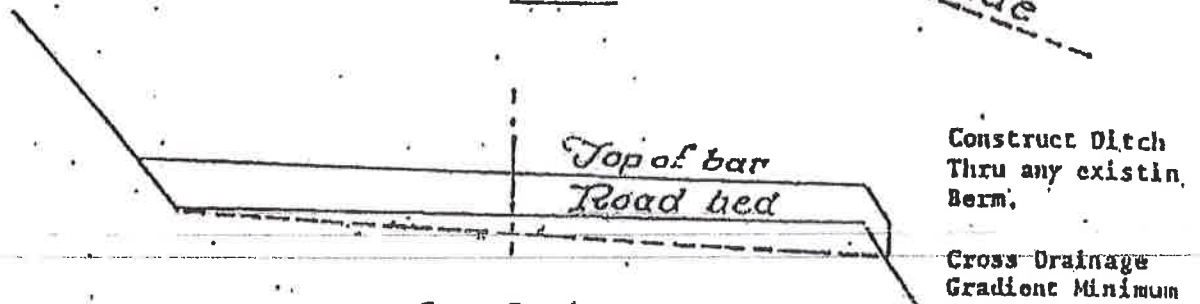
Cross Section
